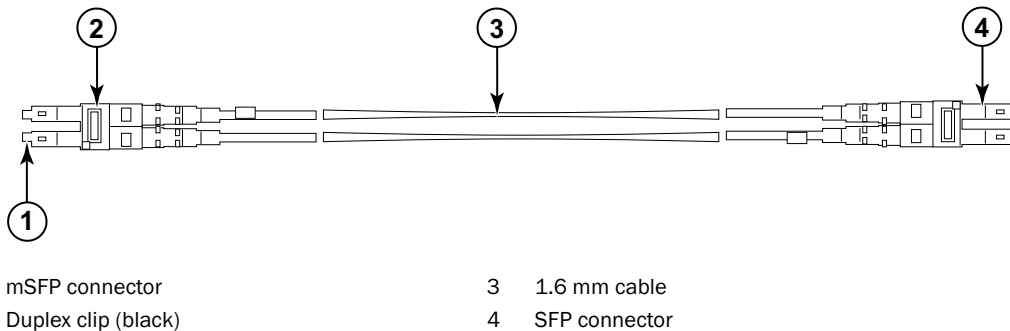
FIGURE 6 Cable design for the mSFP patch cables for the FC8-64 high density port blade
